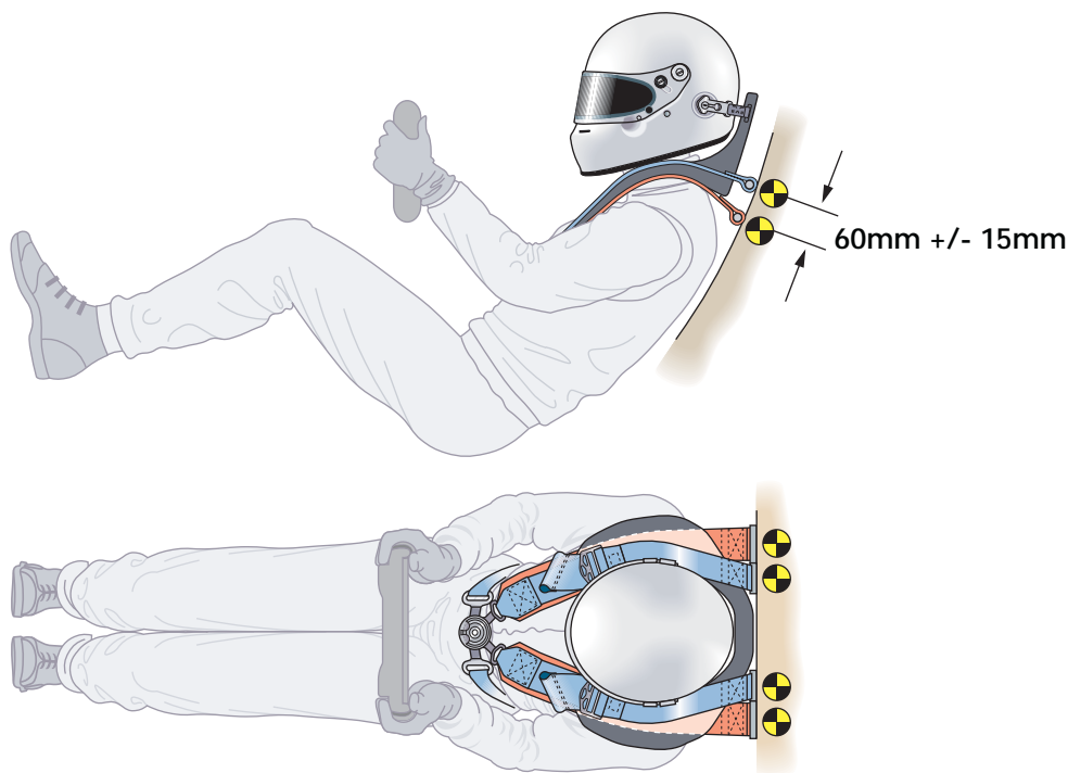
Figure 6. Installation of HANS® double belts in cars where ( X < 200 mm)
